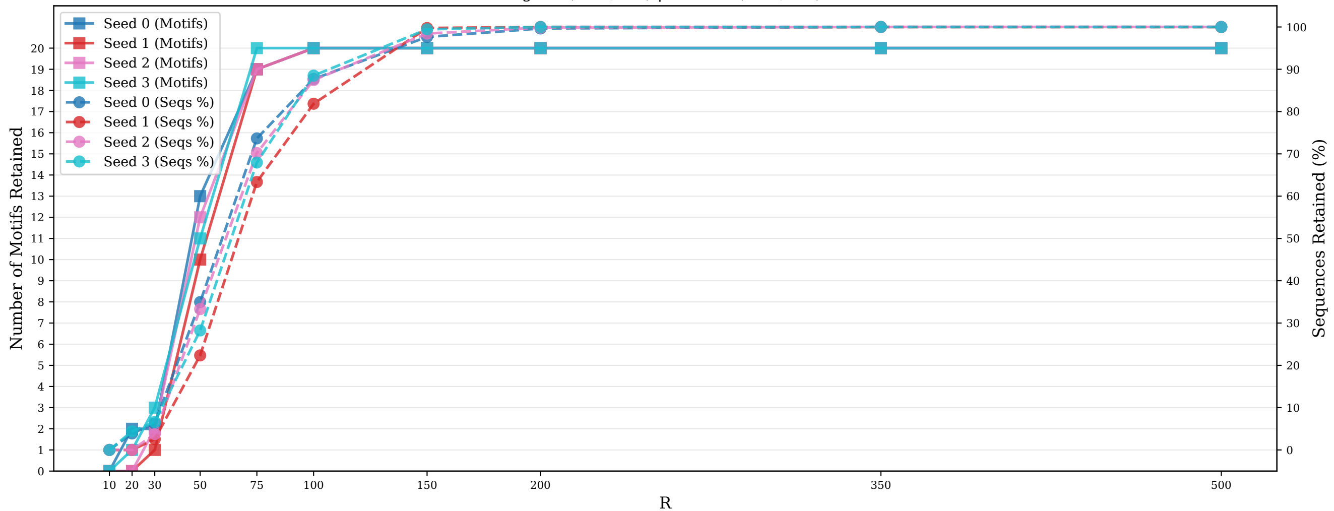
Motif & Sequence Retention vs Neuron Threshold (Multiple Seeds)
